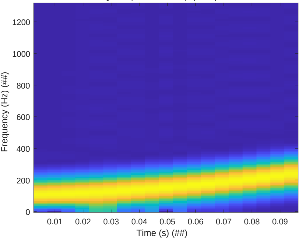
Signal: Quadratic Chirp (#####)
